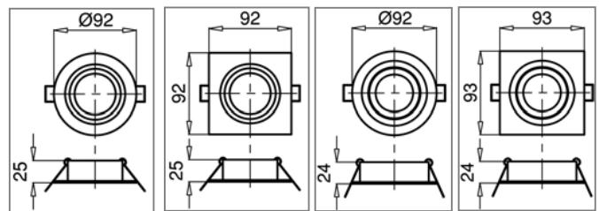
ALU-LED 10105AL/AL
