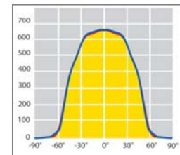
MACH 5 C LED 2x40°
