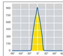
MACH 5 C LED 2x30°
