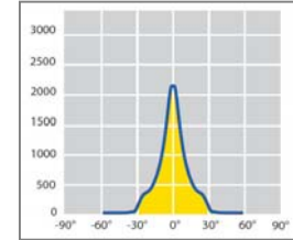
MACH 5 C LED 2x15°
